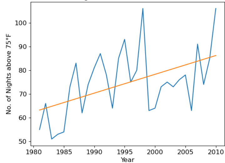
Total Nights Above 75°F (1981-2010)
