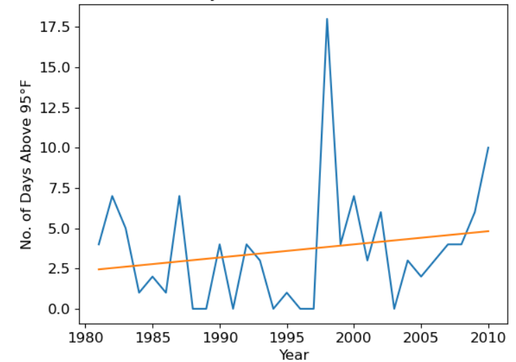
Total Days Above 95°F (1981-2010)
