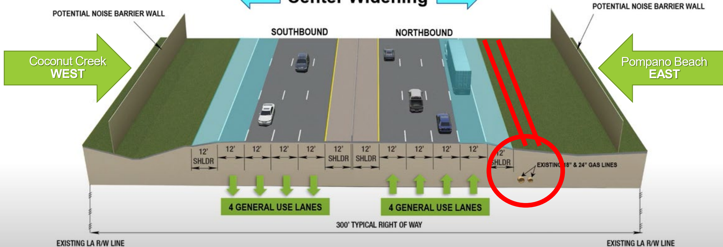
Proposed Typical Section (from 2006 PD&E Study) South of Atlantic Blvd to Hillsboro Blvd
